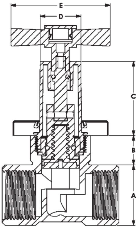
Female Thread
